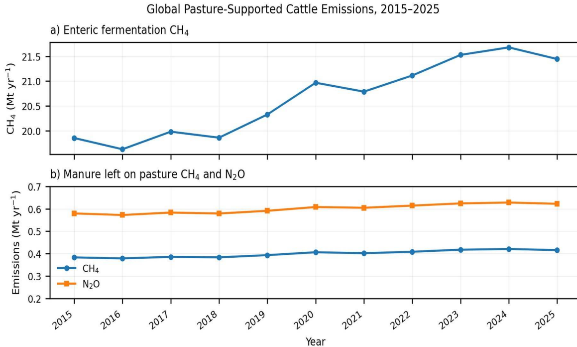
Figure 8 Global Tier 2 emission trends for pasture-supported cattle during 2015-2025. Emissions are reported in megatonnes per year ( \text{Mt yr}^{-1} ). a) Enteric Fermentation \text{CH}_4 emissions. b) Manure left on pasture \text{CH}_4 and \text{N}_2\text{O} emissions.
